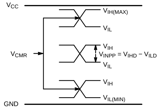
Figure 23. V_{CM} Diagram
