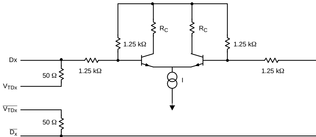
Figure 10. Input Structure
