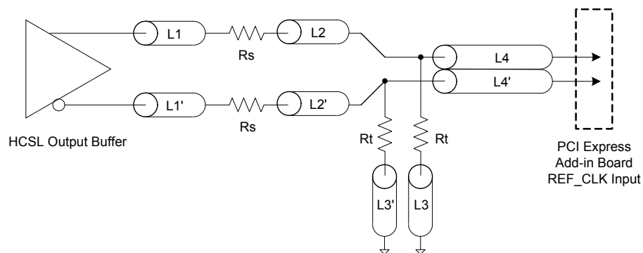
Figure 2: PCI Express Connector Routing
