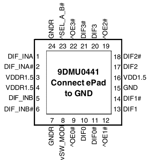
24 VFQFPN, 4x4 mm, 0.5mm pitch
