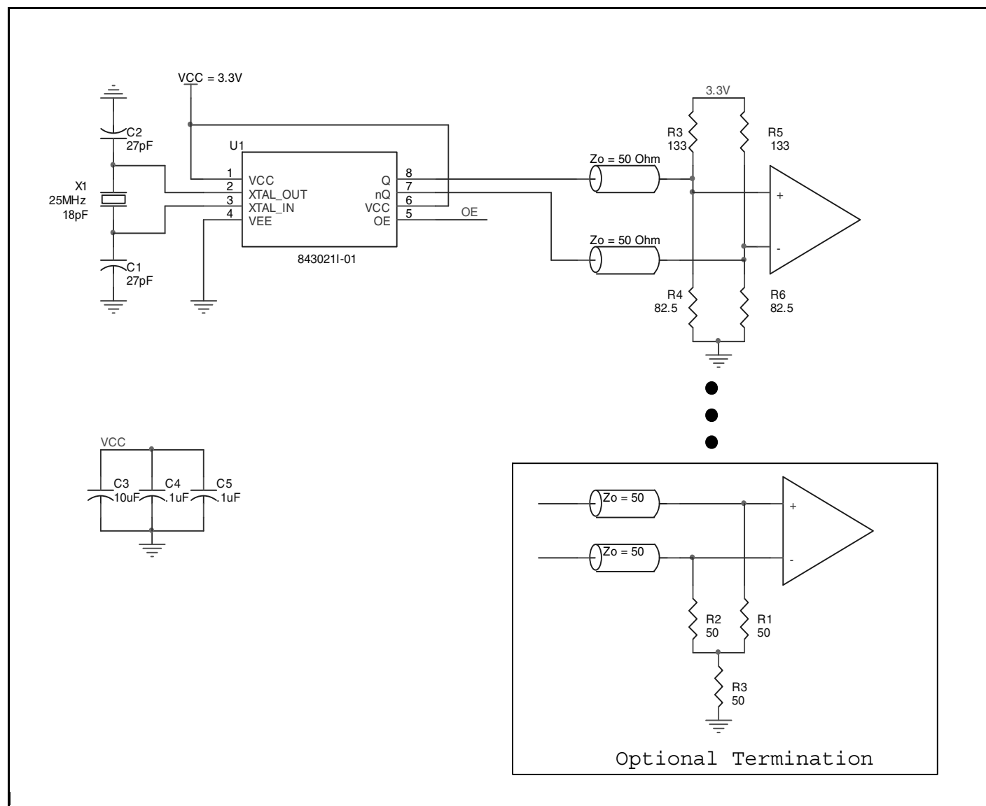
Figure 5. 843021I-01 Schematic Example
