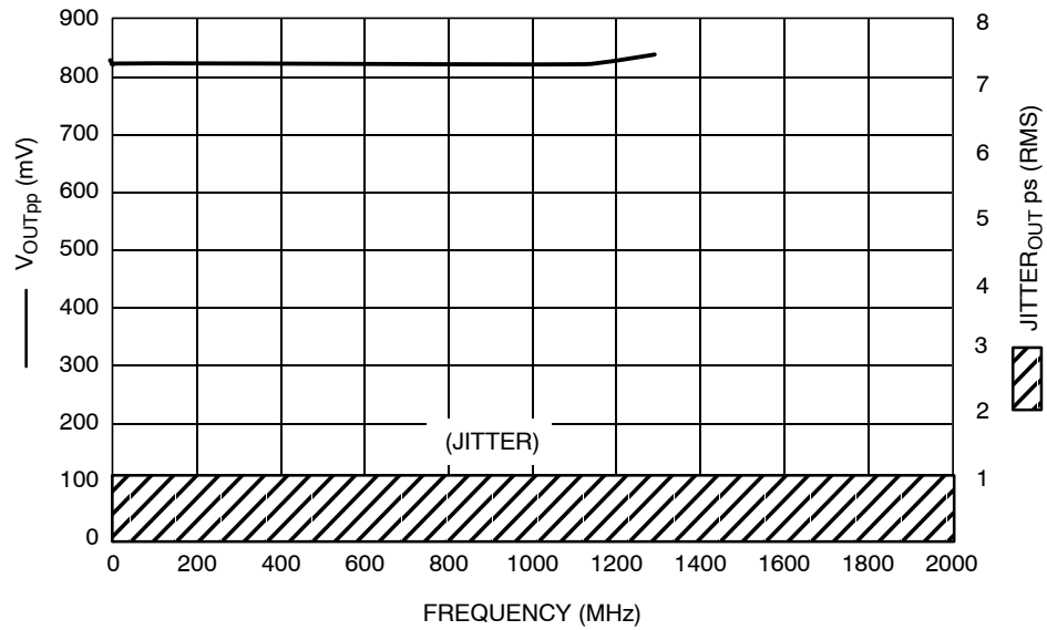
Figure 7. \div 4 , F_{\max}/\text{Jitter}
