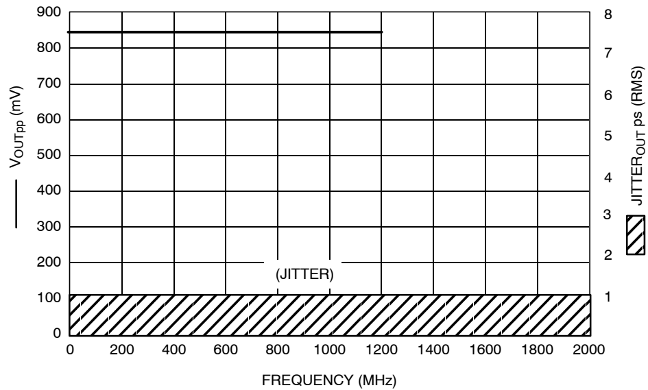
Figure 8. \div 6 , F_{\max}/\text{Jitter}
