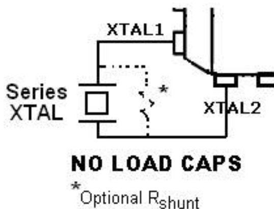
Figure 6. Crystal Application
