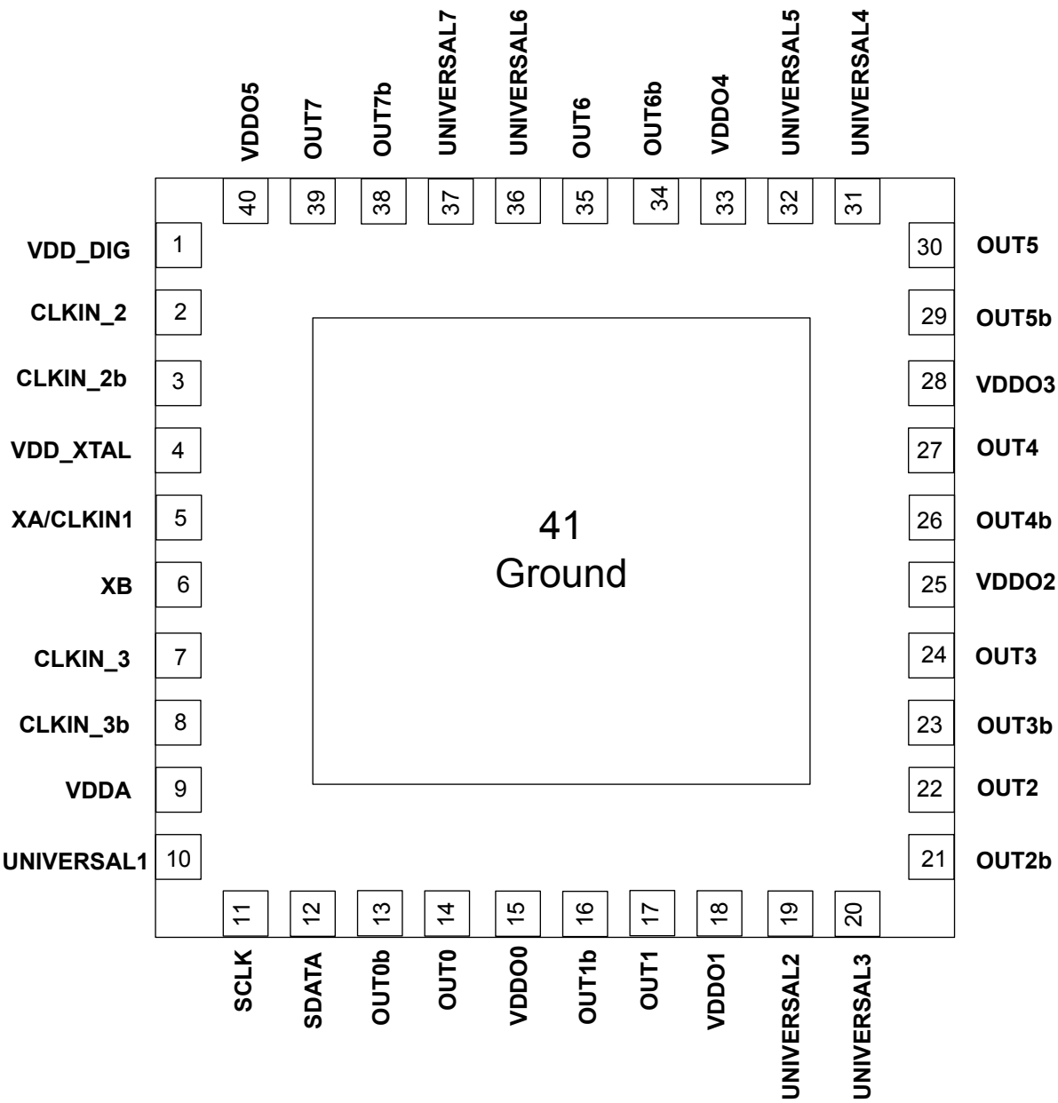
Figure 6.2. 40-QFN
