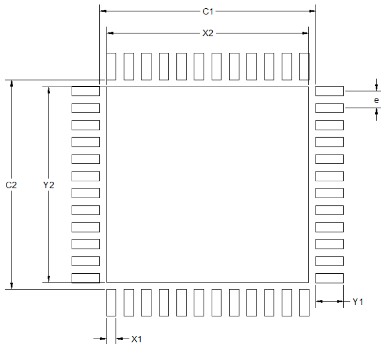
Figure 8.1. 48-QFN Land Pattern
