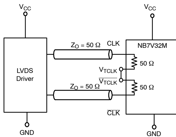
Figure 13. LVDS Interface
