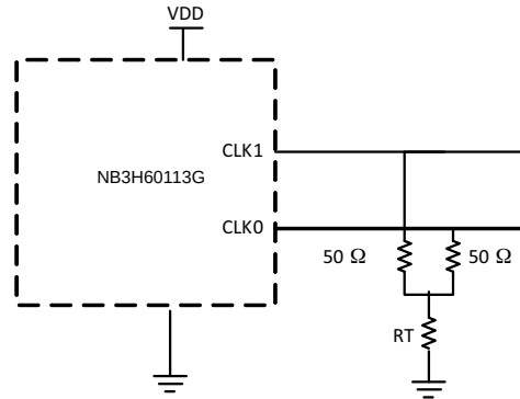
Figure 21. LVPECL Y-Termination
