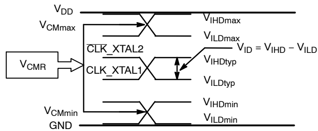
Figure 7. VCMR Diagram
