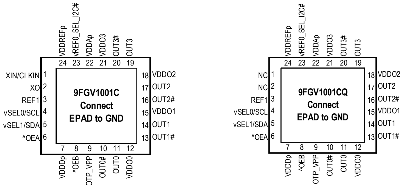
Figure 1. Pin Assignments for 9FGV1001C 4 x 4 mm 24-VFQFPN and 24-LGA Packages – Top View
