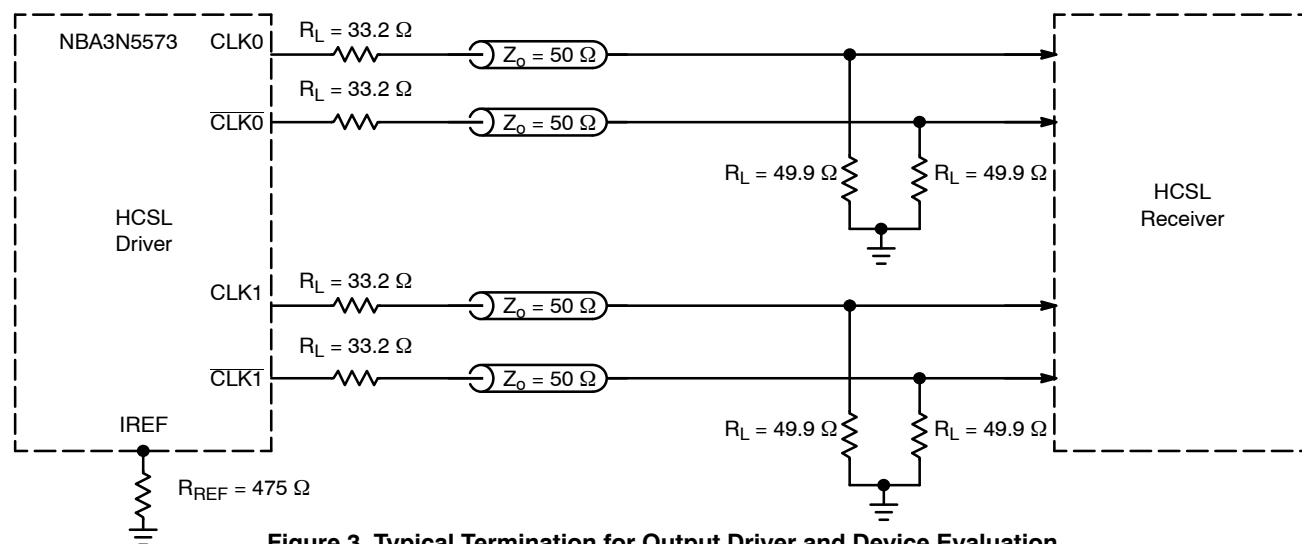
Figure 3. Typical Termination for Output Driver and Device Evaluation
