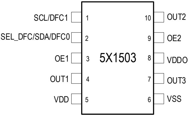
Figure 1. Pin Assignments for 2.0 × 2.0 mm 10-VFQFPN Package
