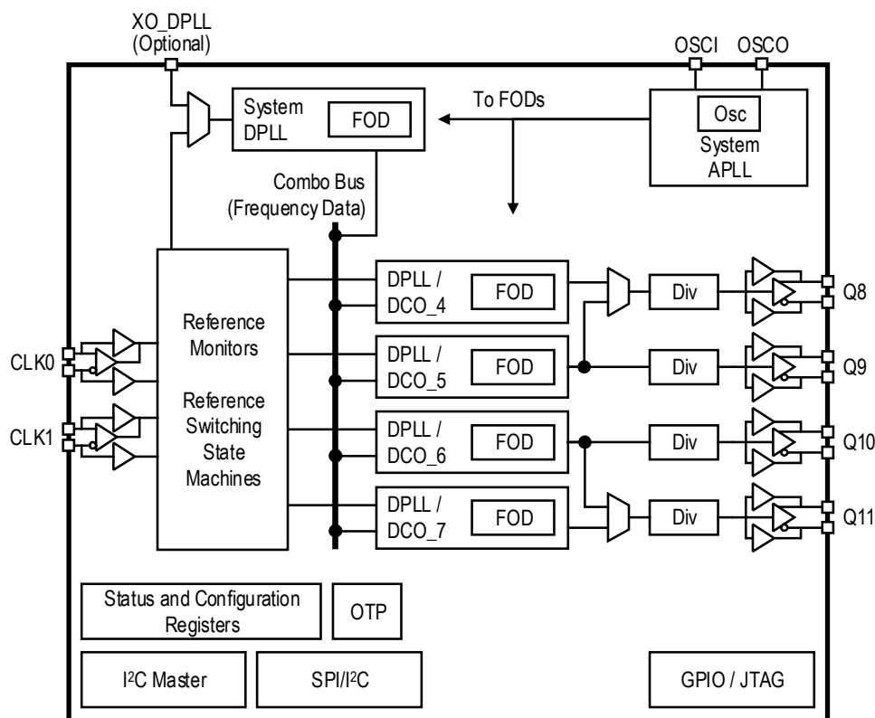
Figure 1. Block Diagram
