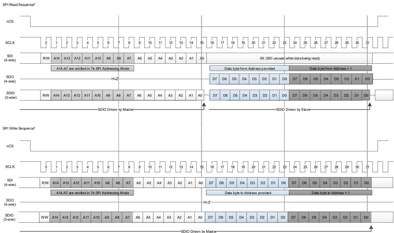
Figure 21. SPI Sequencing
