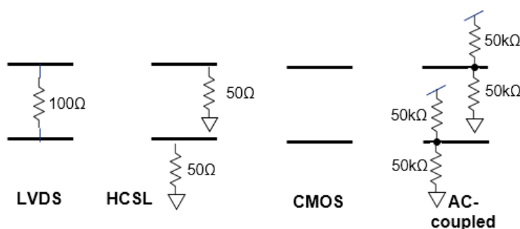
Figure 7. Input Buffer Behavior by Protocol
