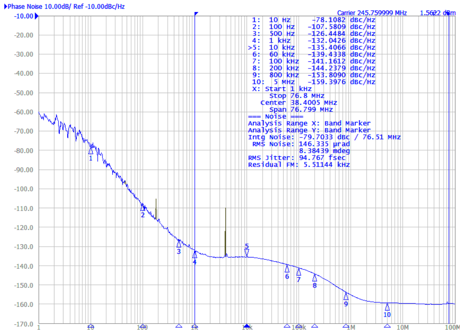
Figure 11. 245.76MHz Output Phase Noise
