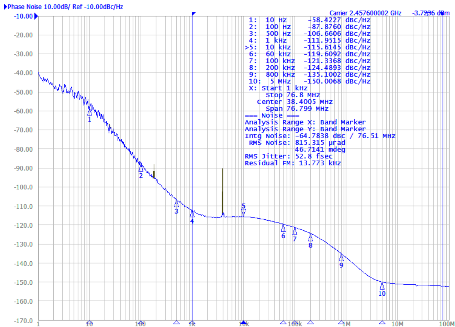
Figure 9. 2457.6MHz Output Phase Noise
