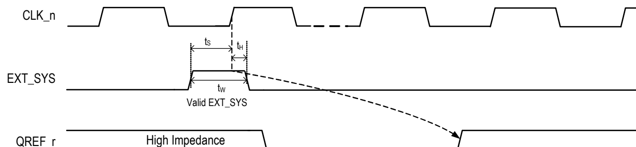
Figure 8. EXT_SYS Input Timing Diagram
