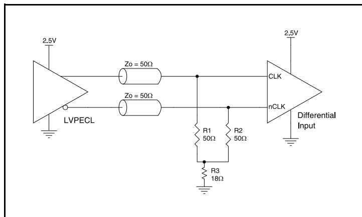
Figure 5B. CLK/nCLK Input Driven by a 2.5V LVPECL Driver
