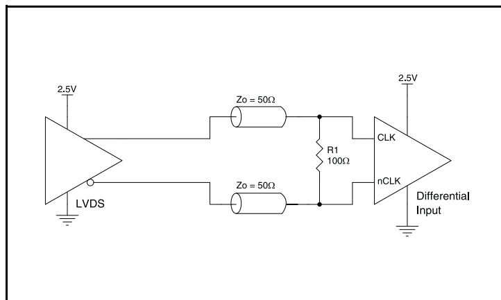
Figure 5D. CLK/nCLK Input Driven by a 2.5V LVDS Driver
