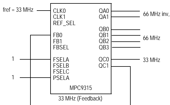
MPC9315 1:1 frequency configuration (feedback of QC1 = 33 MHz). FSELB = PSEL = H. All other control pins are left open.
