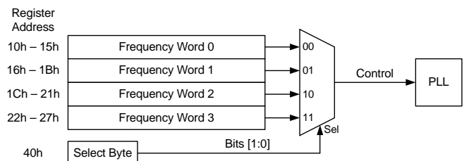
Figure 2. Frequency Words
