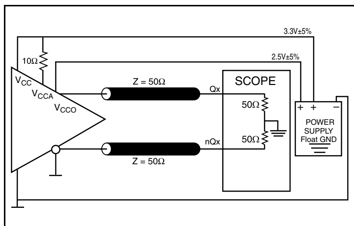
3.3 Core/2.5V LVDS Output Load Test Circuit
