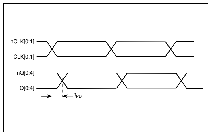
Propagation Delay
