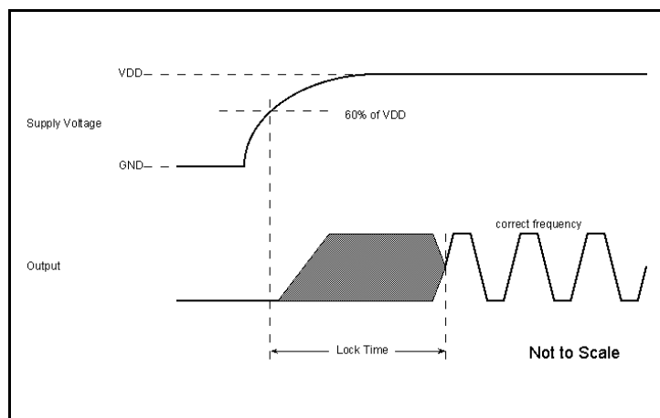
PLL Lock Time
