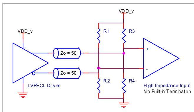
Figure 15. LVPECL Parallel Termination 2
