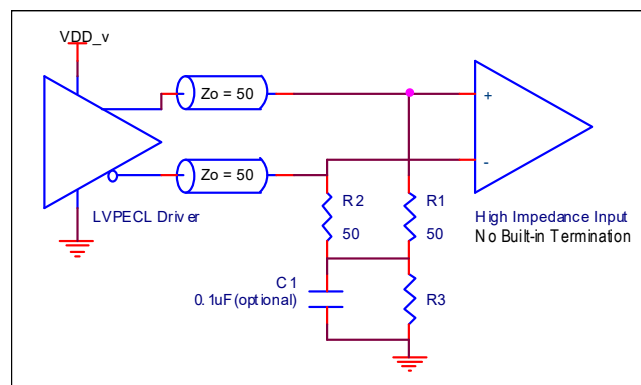
Figure 16. LVPECL Y-Termination
