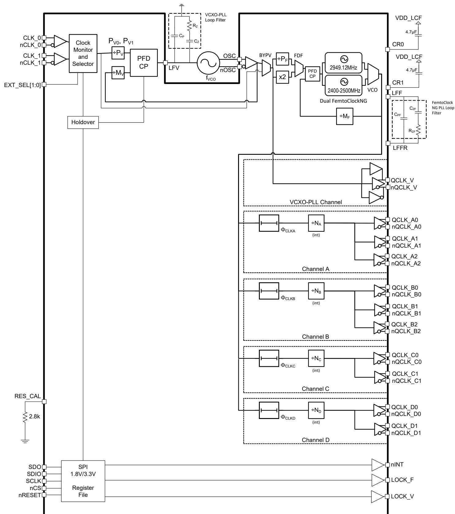
Figure 1. Block Diagram
