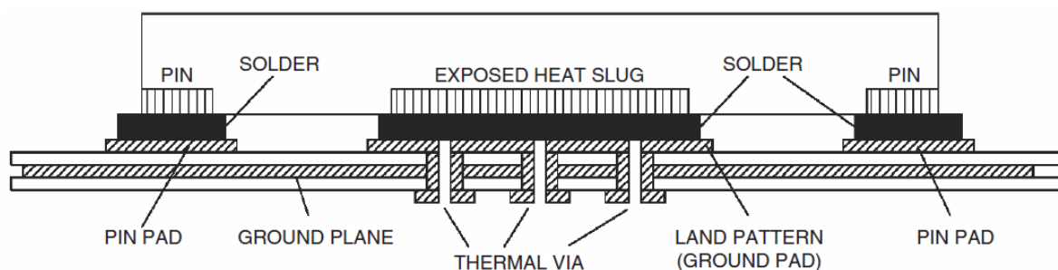
Figure 33. Assembly for Exposed Pad Thermal Release Path - Side View (Drawing not to scale)
