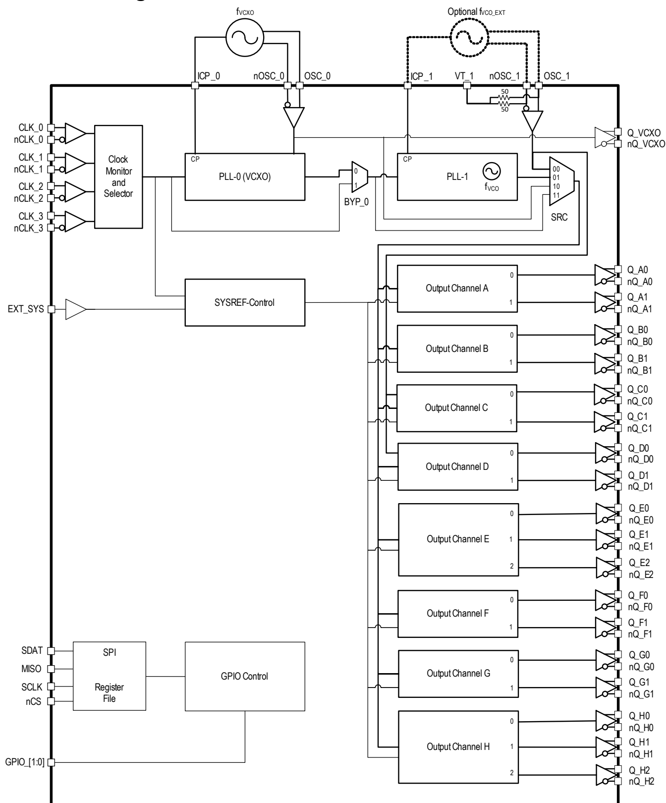
Figure 2. Block Diagram (f VCXO = 3932.16MHz)
