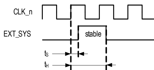
Figure 18. Setup And Hold Time Definition for SRG = 001
