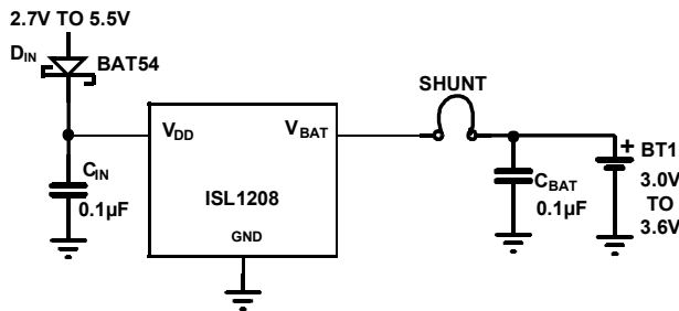
FIGURE 21. POWER GLITCH PROTECTION CIRCUIT
