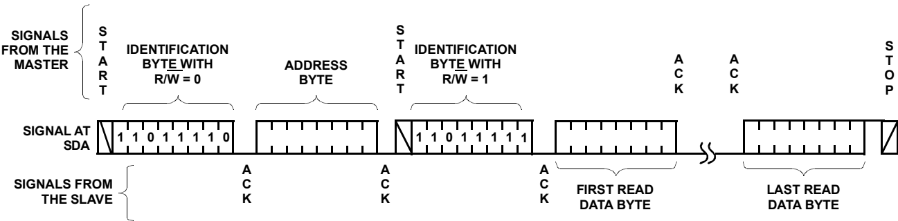
FIGURE 17. READ SEQUENCE
