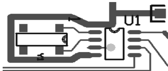
FIGURE 20. SUGGESTED LAYOUT FOR ISL1208 AND CRYSTAL
