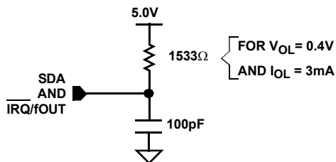
FIGURE 8. STANDARD OUTPUT LOAD FOR TESTING THE DEVICE WITH V_{DD} = 5.0V
