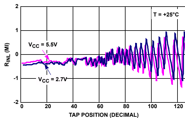
FIGURE 4. INL vs TAP POSITION IN RHEOSTAT MODE FOR 10k \Omega (W)
