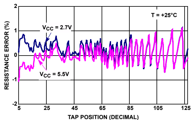
FIGURE 2. RESISTANCE ERROR vs TAP POSITION [ I(RW) = V_{CC}/R_{TOTAL} ] FOR 10k \Omega (W)
