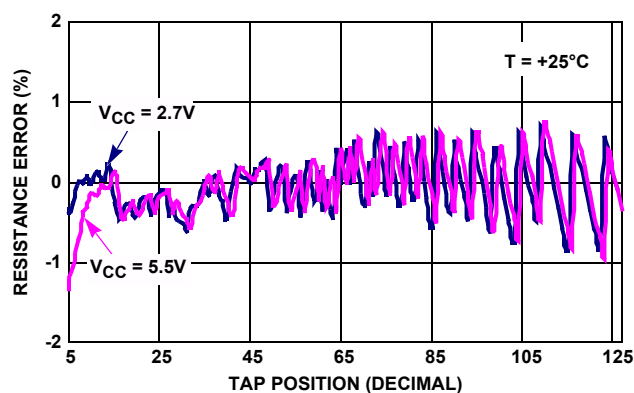
FIGURE 1. RESISTANCE ERROR vs TAP POSITION [ I(RW) = V_{CC}/R_{TOTAL} ] FOR 100k \Omega (T)
