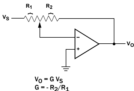
FIGURE 21. INVERTING AMPLIFIER
