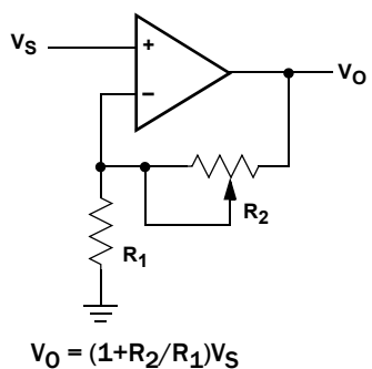
FIGURE 15. NONINVERTING AMPLIFIER
