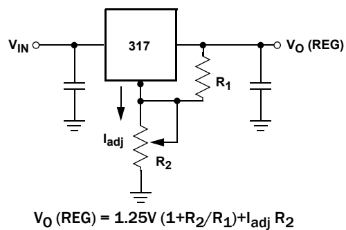
FIGURE 16. VOLTAGE REGULATOR
