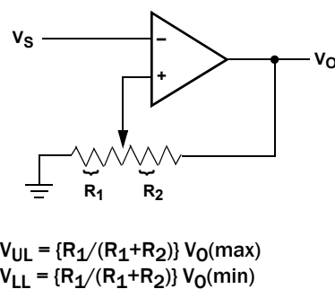
FIGURE 18. COMPARATOR WITH HYSTERESIS
