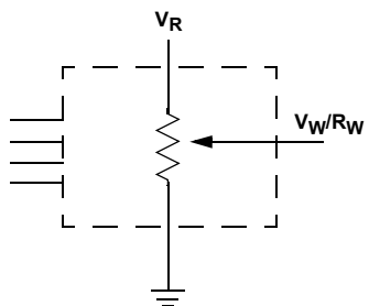
FIGURE 13. THREE TERMINAL POTENTIOMETER; VARIABLE VOLTAGE DIVIDER
