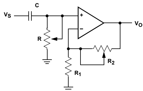
FIGURE 20. FILTER
