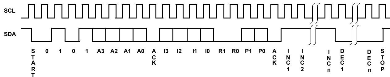
FIGURE 9. INCREMENT/ DECREMENT INSTRUCTION SEQUENCE
