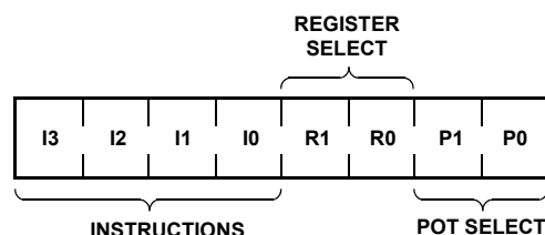
FIGURE 6. INSTRUCTION BYTE FORMAT
