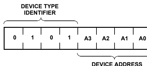
FIGURE 4. SLAVE ADDRESS
