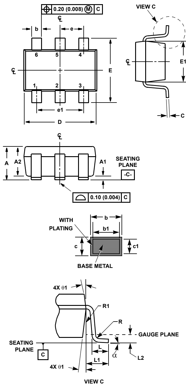
P6.064 6 LEAD SMALL OUTLINE TRANSISTOR PLASTIC PACKAGE
