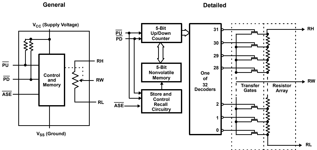
Figure 1. Block Diagrams
