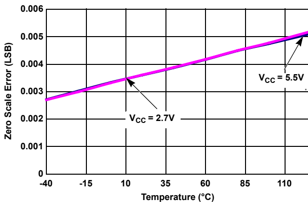
Figure 6. ZS Error vs Temperature
