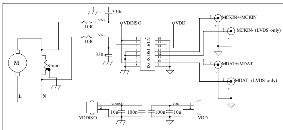
Figure 6. Typical application schematics
