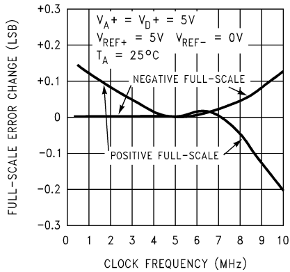
Full-Scale Error Change vs. Clock Frequency
