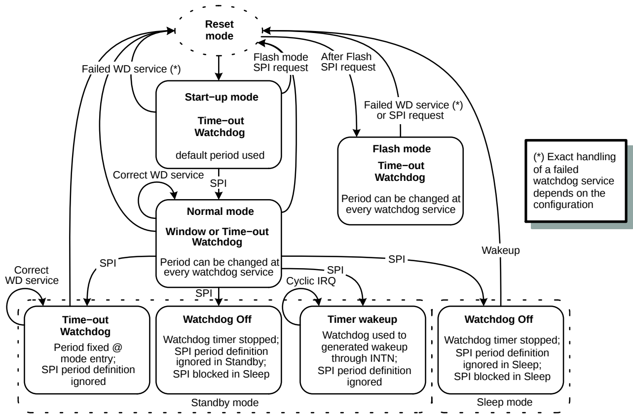
Figure 14. Watchdog Modes
