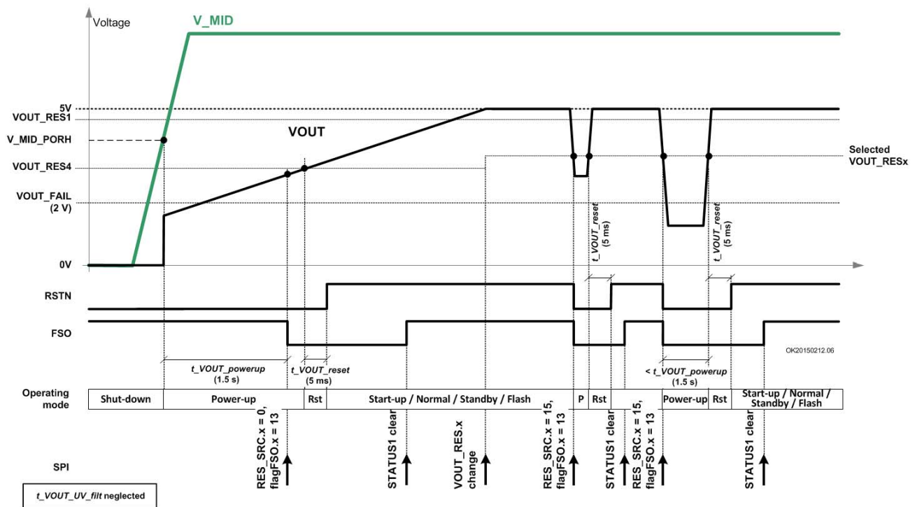
Figure 5. VOUT Monitoring
