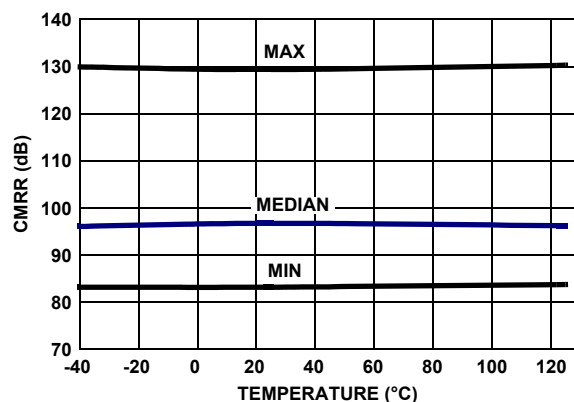
FIGURE 31. CMRR vs TEMPERATURE V_{CM} = -2.5V TO +2.5V , V_+ = 5V , V_- = 0V , R_L = \text{Open} . (Continued)
