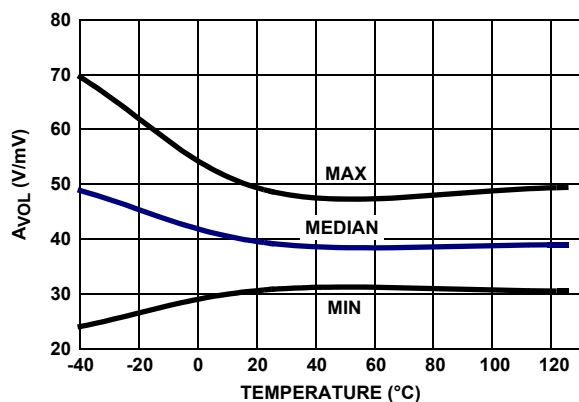
FIGURE 30. A_{VoL} vs TEMPERATURE R_L = 1k , V_+ = 5V , V_- = 0V , V_{CM} = 2.5V , R_L = \text{Open} . (Continued)
