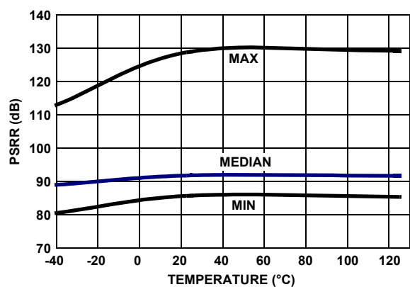
FIGURE 32. PSRR vs TEMPERATURE V_+ = 5V , V_- = 0V , V_{CM} = 2.5V , R_L = \text{Open} . (Continued)
