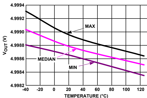
FIGURE 34. V_{OUT} HIGH vs TEMPERATURE R_L = 100k , V_+ = 5V , V_- = 0V , V_{CM} = 2.5V , R_L = \text{Open} . (Continued)
