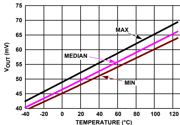
FIGURE 35. V_{OUT} LOW vs TEMPERATURE R_L = 1k , V_+ = 5V , V_- = 0V , V_{CM} = 2.5V , R_L = \text{Open} . (Continued)
