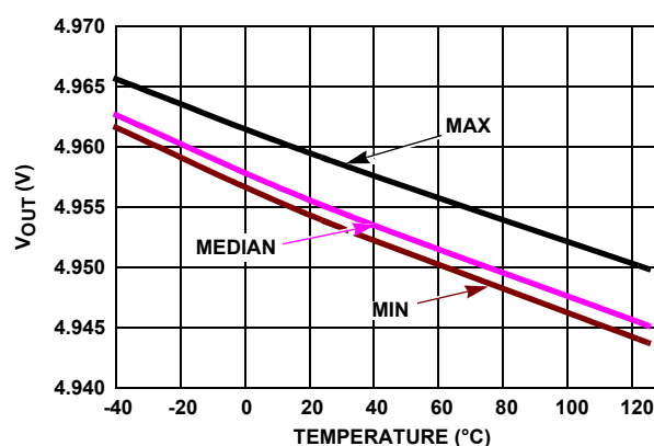
FIGURE 33. V_{OUT} HIGH vs TEMPERATURE R_L = 1k , V_+ = 5V , V_- = 0V , V_{CM} = 2.5V , R_L = \text{Open} . (Continued)
