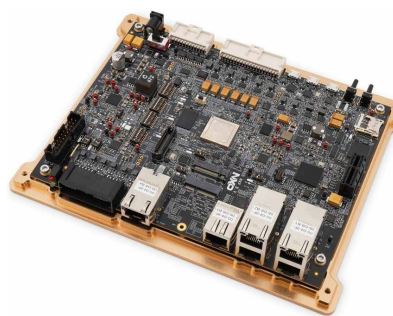
Vehicle network processing reference design board 2
