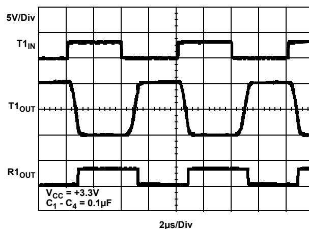
Figure 17. Loopback Test at 250kbps
