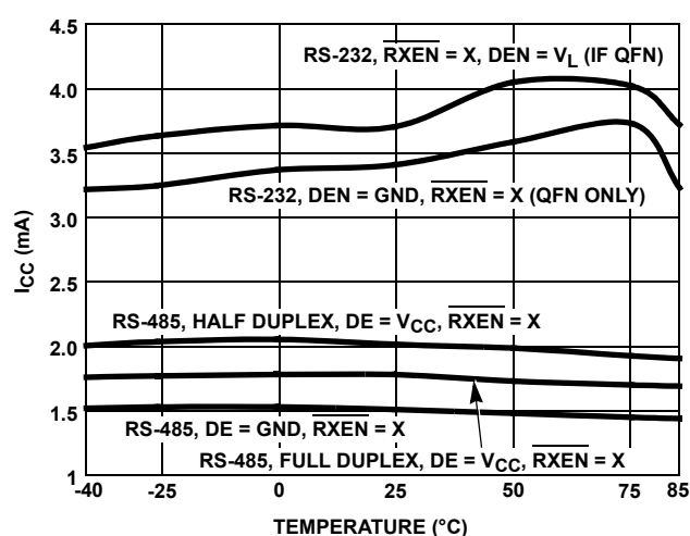
FIGURE 19. SUPPLY CURRENT vs TEMPERATURE
