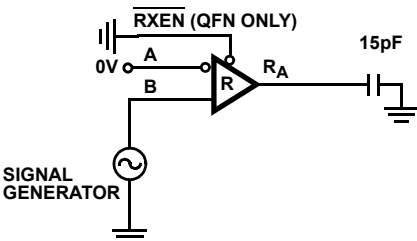
FIGURE 12A. TEST CIRCUIT
