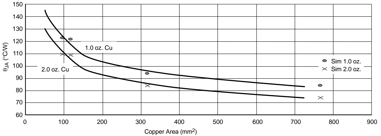
Figure 22. SOIC-14, \theta_{\text{JA}} as a Function of the Pad Copper Area Including Traces, Board Material
