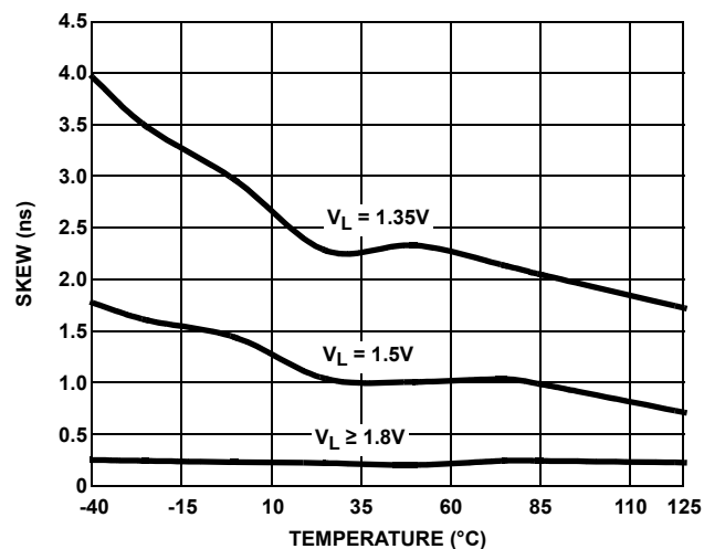
FIGURE 14. DRIVER DIFFERENTIAL SKEW vs TEMPERATURE
