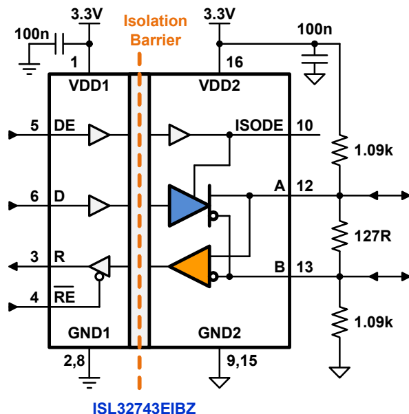
Figure 2. Typical Operating Circuit
