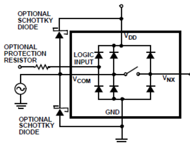
Figure 11. Overvoltage Protection
