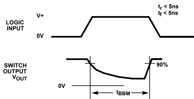
FIGURE 1. SWITCHING TIMES
