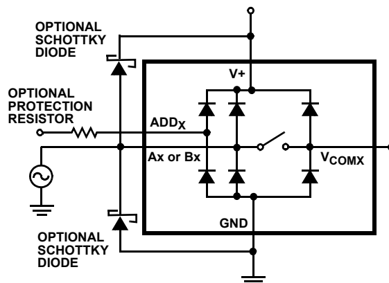
FIGURE 7. OVERVOLTAGE PROTECTION
