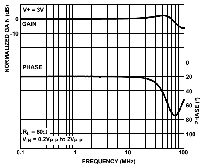
FIGURE 12. FREQUENCY RESPONSE
