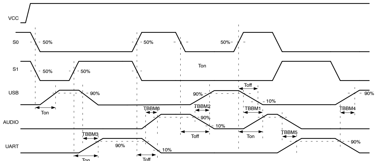
Figure 8. Timing Waveforms
