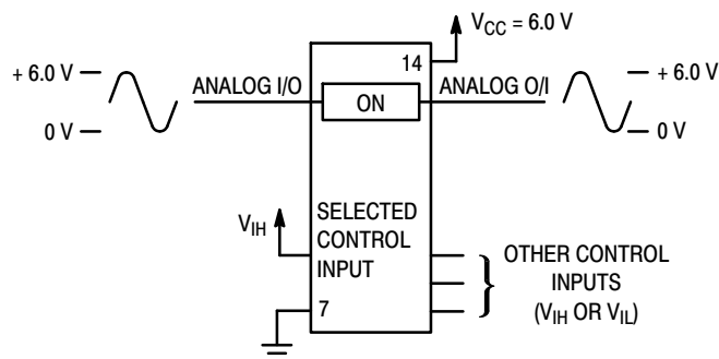
Figure 16. 6.0 V Application
