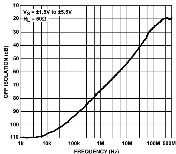
FIGURE 16. OFF ISOLATION
