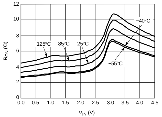
Figure 13. R_{ON} vs. V_{IN} vs. Temperature @ V_{CC} = 4.5 V
