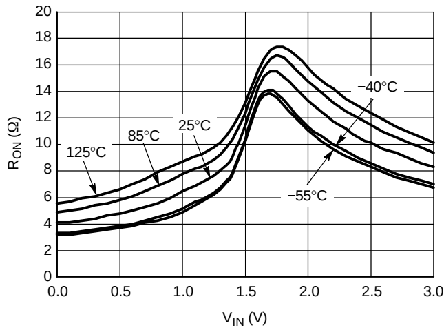
Figure 12. R_{ON} vs. V_{IN} vs. Temperature @ V_{CC} = 3.0 V
