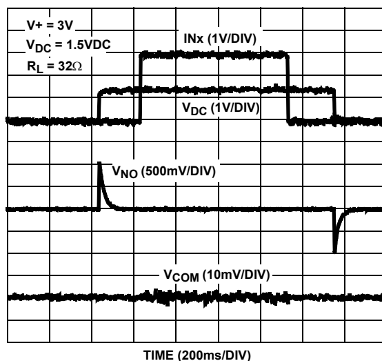
FIGURE 24. CLICK AND POP ELIMINATION 32Ω LOAD 200ms DELAY
