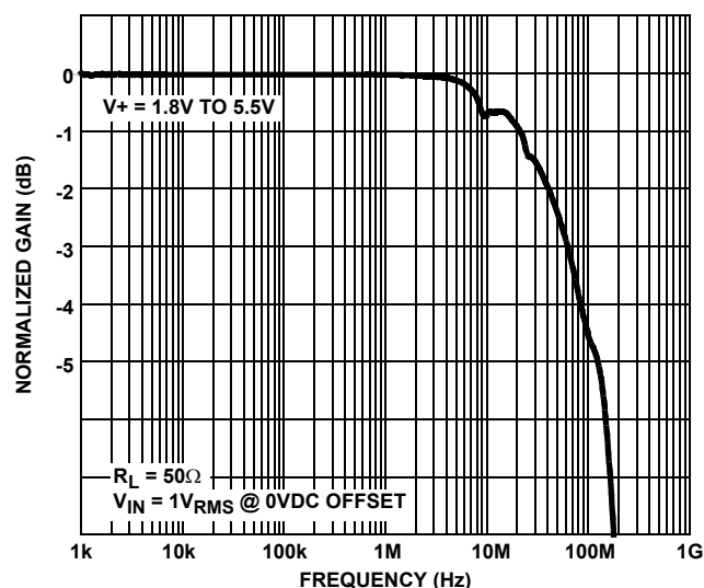
FIGURE 21. FREQUENCY RESPONSE
