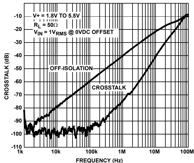
FIGURE 22. CROSSTALK AND OFF ISOLATION
