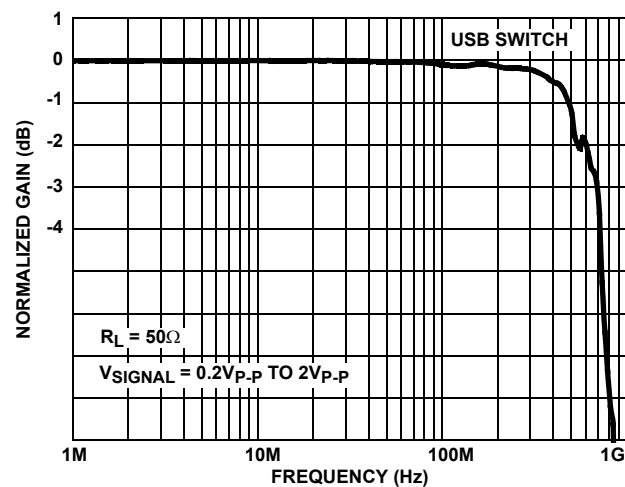
FIGURE 27. FREQUENCY RESPONSE
