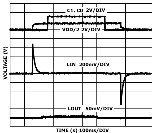
FIGURE 31. 1\text{k}\Omega AC COUPLED CLICK/POP REDUCTION
